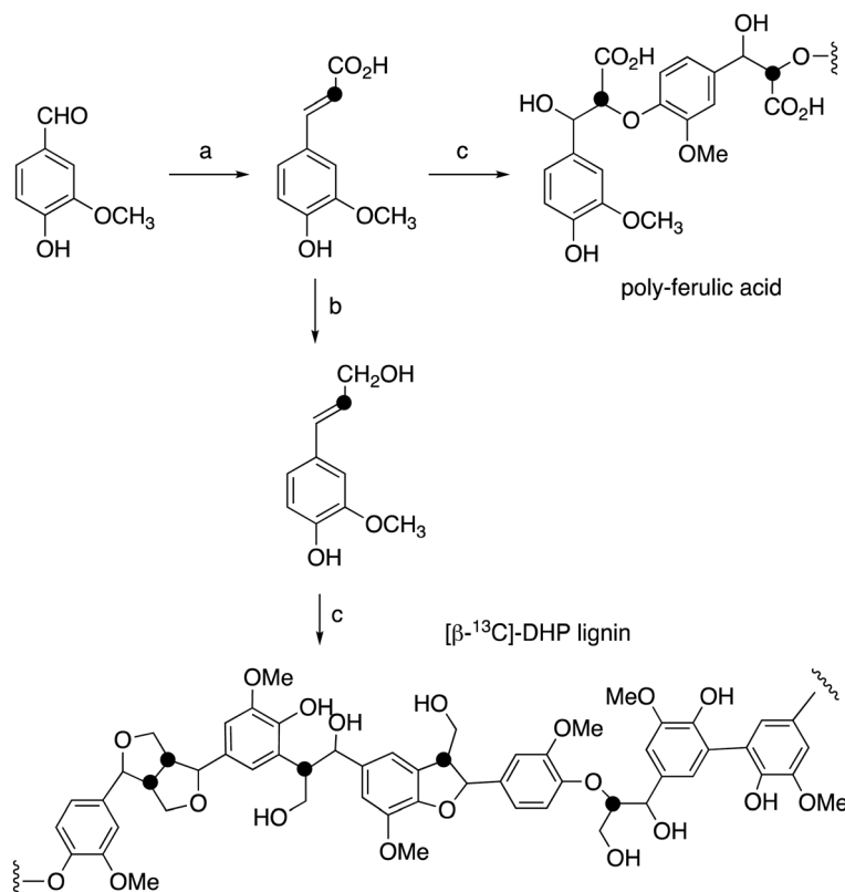
Fig. 2 Synthetic route for preparation of [ \beta - ^{13}\text{C} ]-coniferyl alcohol, [ \beta - ^{13}\text{C} ]-DHP lignin, and [ \beta - ^{13}\text{C} ]-polyferulic acid. (a) [ ^{13}\text{C} ]-Malonic acid, pyridine, aniline, 86%; (b) Nocardia iowensis carboxylic acid reductase (NiCAR), Coptotermes gestroi aldo-keto reductase (CgAKR-1), yield 70%; (c) horseradish peroxidase.
