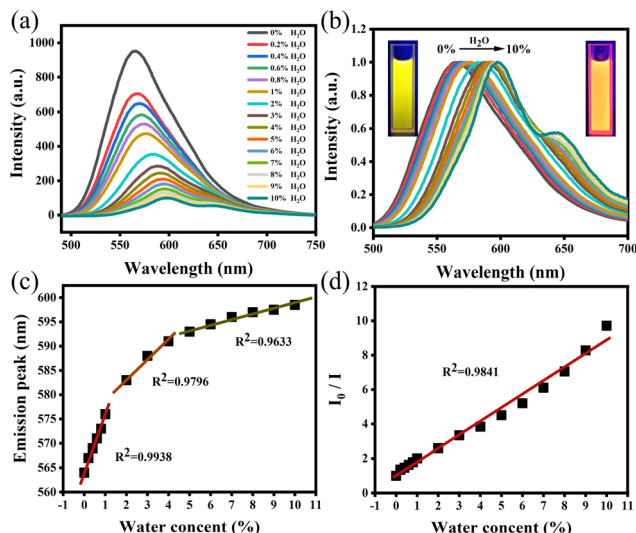
Fig. 3 (a) Fluorescence spectra of O-CDs in acetone with different water contents. (b) Normalized fluorescence spectra. Illustrations are photos of solutions with 0% and 10% water content under UV light. (c and d) Fitting of maximum emission peak and I_0/I .
