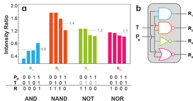
Fig. 11 (a) Bar chart of the intensity ratios R1–R4 as a function of the temperature input (T) and excitation power density (P 0 ) presenting the corresponding threshold (pointed line) the truth tables in the bottom. (b) Schematic representation of the logic circuitry with the logic gates presented in (a). Figure reproduced from ref. 81.
