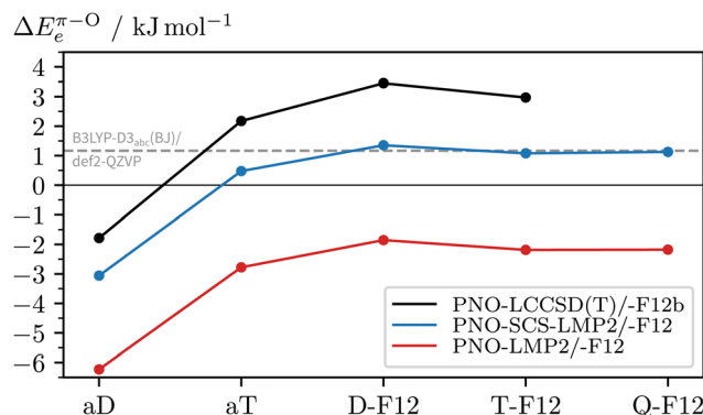
Fig. 9 Comparison of PNO (with aX≡aVXZ) and PNO-F12 (with X-F12≡VXZ-F12) predictions of the relative electronic stabilities of c2NA_O and c2NA_\pi ( \Delta E_e^{\pi-O} ) for increased coverage of the one-particle basis space. The optimised B3LYP-D3 abc (BJ)/def2-QZVP geometries are used (reference values shown in grey).
