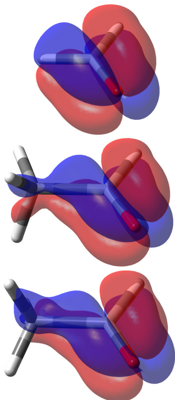
Fig. 9 Specific rotation power density, [\Phi]_\text{D}(\mathbf{r}) : top formaldehyde; middle acetaldehyde with achiral conformation; bottom acetaldehyde with chiral conformation. Calculated at B3LYP/aug-cc-pVTZ level of theory. Iso-surfaces are \pm 100 \text{ deg}[\text{dm g cm}^{-3}]^{-1} a_0^{-3} , red/blue positive/negative.
