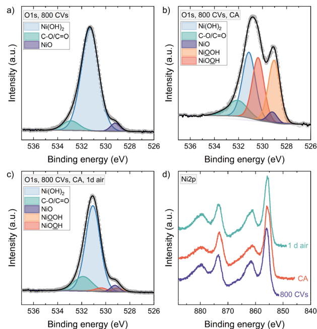
Fig. 4 XPS spectra of the fitted O1s and Ni2p regions of a 6 nm NiO thin film after an activation treatment of 800 CVs. a) with 800 CVs, NiO was almost completely transformed to \text{Ni}(\text{OH})_2 . b) after CA at 1.55 V vs. RHE, NiOOH is detected. c) Keeping the portion of the NiO peak constant in the fitting of the O1s region, little NiOOH is needed to fit the spectrum after storing the sample for one day in atmospheric conditions. d) Ni2p lines after 800 CVs, CA, and storage in air.
