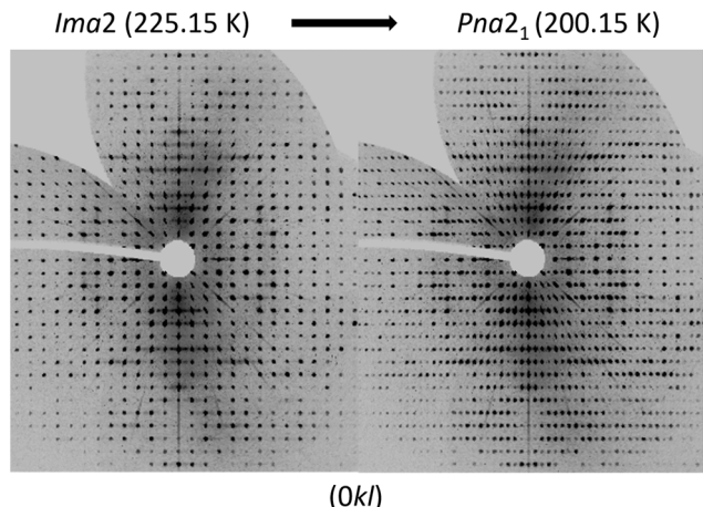
Fig. 6 Digitally generated precession images of the (0kl) plane of UoC-9(Ca) from single crystal X-ray diffraction data (Mo-K \alpha ) recorded at 225.15 K (left) and 200.15 K (right).
