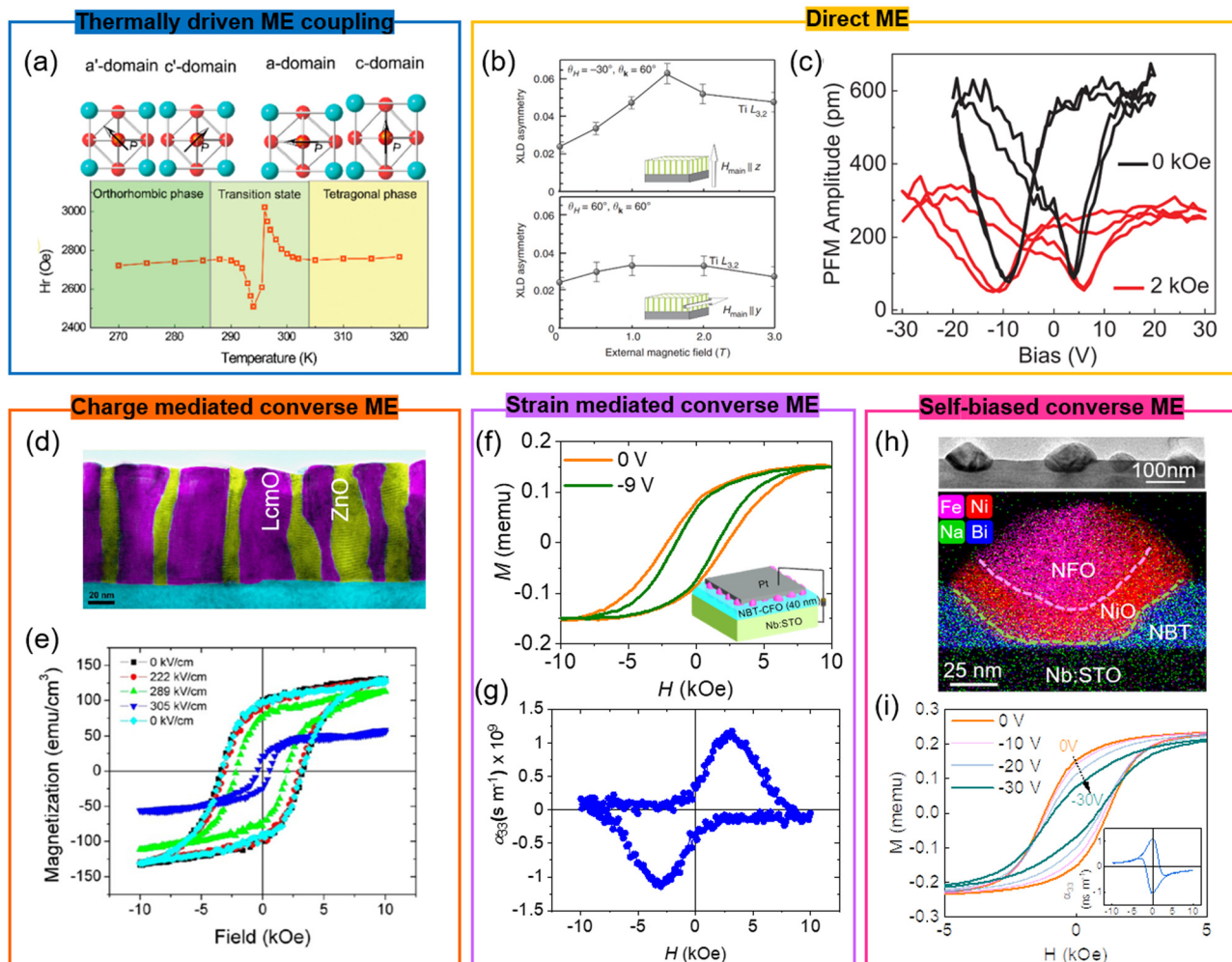
Fig. 8 Enhanced magnetoelectric properties achieved using VAN structures. (a) Thermally-driven ME effect in \text{Y}_3\text{Fe}_5\text{O}_{12}\text{-BaTiO}_3 VAN films detected by the FMR. Reproduced with permission. 137 Copyright 2017 American Chemical Society. (b) XLD asymmetry study of the lattice distortion induced by magnetic field in a \text{BaTiO}_3\text{-CoFe}_2\text{O}_4 VAN film, the upper plot showing magnetic field applied OOP and the lower plot showing the magnetic field applied IP. Reproduced with permission. 138a Copyright 2013 Springer Nature. (c) The effect of the application of IP magnetic field on the amplitude–voltage butterfly loop (DME effect) in \text{BaTiO}_3\text{-CoFe}_2\text{O}_4 VAN films. Reproduced with permission. 138b Copyright 2019 Wiley-VCH. (d and e) Charge mediated ME to give the CME effect in \text{La}_2\text{CoMnO}_6\text{-ZnO} VAN film. Reproduced with permission. 142 Copyright 2013 American Chemical Society. (d) Cross-sectional (false-colour) TEM image of the \text{La}_2\text{CoMnO}_6\text{-ZnO} VAN film. (e) Electric field dependence of the magnetic hysteresis loops of \text{La}_2\text{CoMnO}_6\text{-ZnO} VAN film where the magnetic field is applied IP. (f) In situ electric field control of magnetization (CME effect) in \text{Na}_{0.5}\text{Bi}_{0.5}\text{TiO}_3\text{-CoFe}_2\text{O}_4 VAN film where the magnetic field is applied OOP. Reproduced with permission. 143 Copyright 2018 American Chemical Society. The inset shows a schematic of the application of an in situ electric field. (g) The magneto-electric coefficient of the \text{Na}_{0.5}\text{Bi}_{0.5}\text{TiO}_3\text{-CoFe}_2\text{O}_4 VAN film calculated from the magnetic hysteresis loops given in (f). (h) Cross-sectional TEM and EDX image of a 50 nm-thick \text{Na}_{0.5}\text{Bi}_{0.5}\text{TiO}_3\text{-NiO-NiFe}_2\text{O}_4 film. Reproduced with permission. 40 Copyright 2021 Springer Nature. (i) In situ electric field control of magnetization (CME effect) in a 200 nm-thick \text{Na}_{0.5}\text{Bi}_{0.5}\text{TiO}_3\text{-NiO-NiFe}_2\text{O}_4 VAN film where the magnetic field is applied OOP. The inset shows the magneto-electric coefficient, calculated from the magnetic hysteresis loops. Reproduced with permission. 40 Copyright 2021 Springer Nature.
