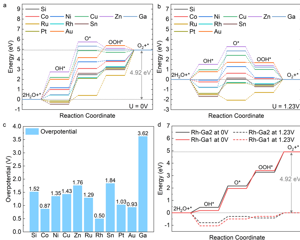
Fig. 2 The free energy diagrams for OER on all doping structures and clean (100) \beta\text{-Ga}_2\text{O}_3 facet at (a) zero cell potential ( U = 0 V), and (b) the equilibrium potential ( U = 1.23 V). (c) The overpotential of all doping elements. (d) The free energy diagrams for Rh-Ga2 and Rh-Ga1 at U = 0 and 1.23 V.
