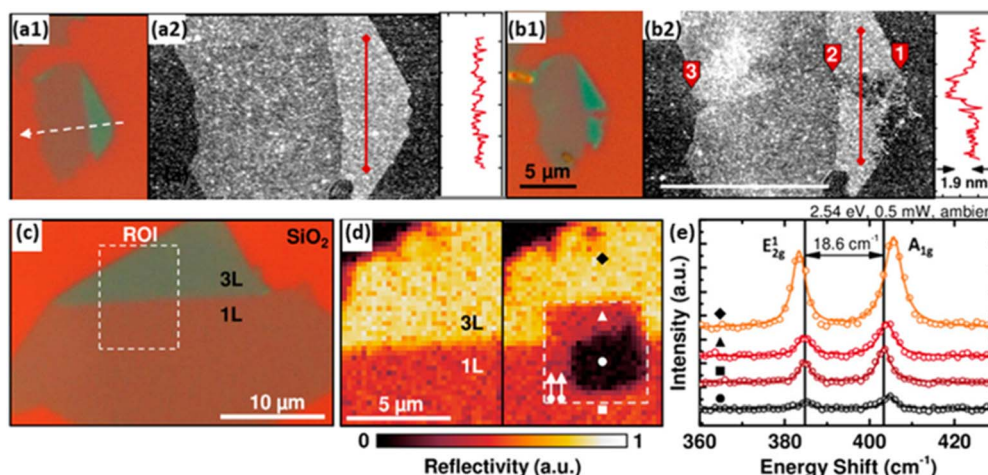
Fig. 5 (a1 and b1) Optical microscopy (100×) and (a2 and b2) AFM images of exfoliated single- and trilayer flake of MoS 2 on a Si/SiO 2 substrate before (top) and after (bottom) laser line scan immersed in the electrolyte. (c) Optical microscopy image (100×) of exfoliated single- (1L) and trilayer (3L) MoS 2 on a Si/SiO 2 substrate. (d) Monochromatic reflectivity map of before (left) and after (right) a laser scan in the electrolyte of the region of interest (ROI) defined in (c). (e) Raman spectra of the spots marked in (d) of untreated, unaffected, and photodegraded regions. Reprinted with permission from ref. 61, copyright 2015, American Chemical Society.
