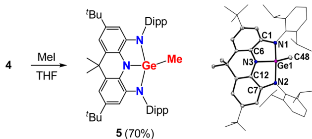
Fig. 5 Left: Reactivity of 4 with methyl iodide. Right: Solid-state structure of 5 (right). The t\text{Bu} and Dipp groups are simplified as wireframes and hydrogen atoms are omitted for clarity. Thermal ellipsoids are set at the 30% probability level. Selected bond lengths ( \text{\AA} ) and angles ( ^\circ ): Ge1–C48 1.9281(18), Ge1–N1 1.8908(15), Ge1–N2 1.8901(15), Ge1–N3 1.8425(14), C1–N1 1.409(2), C7–N2 1.412(2), C6–N3 1.401(2), C12–N3 1.399(2), C1–C6 1.392(2), C7–C12 1.396(2), N1–Ge1–C48 105.00(7), N2–Ge1–C48 104.84(7), N3–Ge1–C48 105.00(7), N1–Ge1–N2 141.84(6), N1–Ge1–N3 86.14(6), N2–Ge1–N3 86.59(6).
