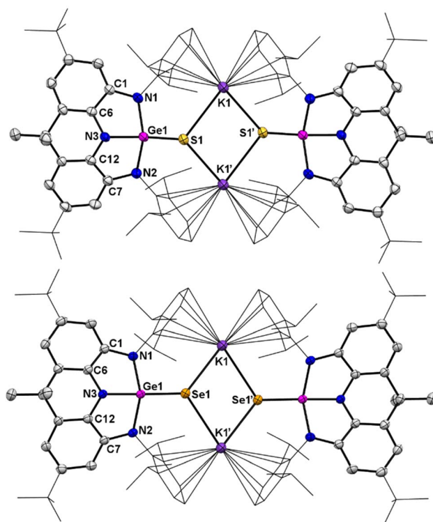
Fig. 6 Top: Solid-state structure of 6. Bottom: Solid-state structure of 7. The t\text{Bu} and Dipp groups are simplified as wireframes and hydrogen atoms are omitted for clarity. Thermal ellipsoids are set at the 30% probability level. Selected bond lengths ( \text{\AA} ) and angles ( ^\circ ) for 6: Ge1–S1 2.1097(8), Ge1–N1 1.917(3), Ge1–N2 1.916(3), Ge1–N3 1.857(3), K1–S1 3.1094(11), K1–S1' 3.1491(10), C1–N1 1.394(4), C1–C6 1.394(4), C7–N2 1.396(4), C7–C12 1.395(4), C12–N3 1.403(4), N3–Ge1–S1 142.98(8), N1–Ge1–N2 139.16(11), N1–Ge1–N3 84.41(10), N2–Ge1–N3 84.41(10). Selected bond lengths ( \text{\AA} ) and angles ( ^\circ ) for 7: Ge1–Se1 2.2595(12), Ge1–N1 1.928(3), Ge1–N2 1.934(3), Ge1–N3 1.872(3), K1–Se1 3.2541(17), K1–Se1' 3.2477(17), C1–N1 1.410(4), C1–C6 1.399(4), C7–N2 1.406(4), C6–N3 1.395(3), C12–N3 1.400(3), C7–C12 1.401(4), N3–Ge1–Se1 143.51(8), N1–Ge1–N2 140.30(11), N1–Ge1–N3 84.52(10), N2–Ge1–N3 83.59(10).
