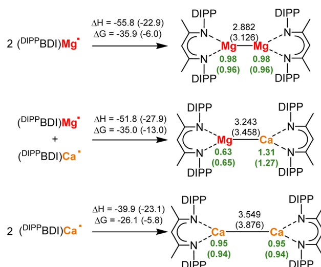
Scheme 2 Formation of homo- and hetero-metallic (^{\text{DIPP}}\text{BDI})\text{Ae}^{\text{DIPP}}\text{BDI} complexes (Ae = Mg or Ca). Enthalpies and Gibbs free energies at 298 K in kcal mol −1 , Ae–Ae distances in Å and NPA charges in green; B3PW91/def2TZVP//def2SVP with dispersion correction (GD3BJ). Values in brackets relate to calculations without dispersion corrections.
