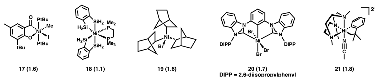
Fig. 9 Structurally characterized formally \text{Ni}^{\text{IV}} complexes investigated by experimentally-calibrated DFT calculations. Ni 3d-vacancies from the calculations are given in parentheses.
