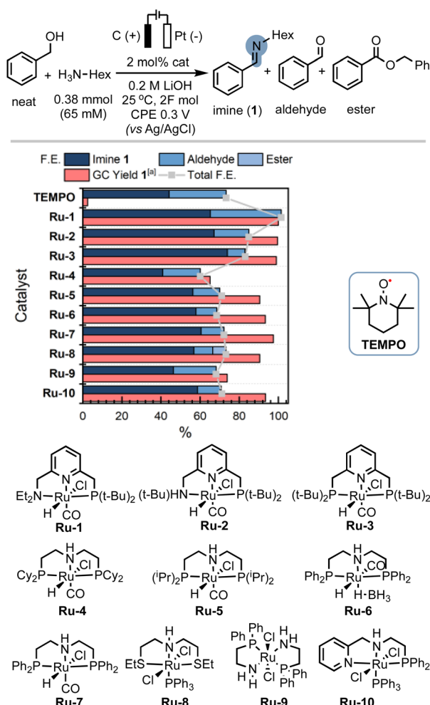
Scheme 2 Ligand effects for the electrocatalytic alcohol oxidation with common metal–ligand cooperative catalysts. [a] GC-MS yield with mesitylene as an internal standard. The amount of imine formation from benzyl alcohol auto-oxidation is subtracted from the product distribution and the yield is corrected for the initial presence of benzaldehyde (see ESI Section 3†).
