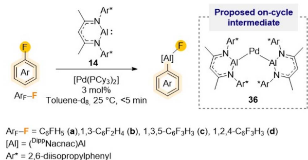
Scheme 11 Palladium-catalysed C–F alumination of fluoroarenes using Roesky's Al(I) ( 14 ) and [Pd(PCy 3 ) 2 ] as pre-catalyst.
