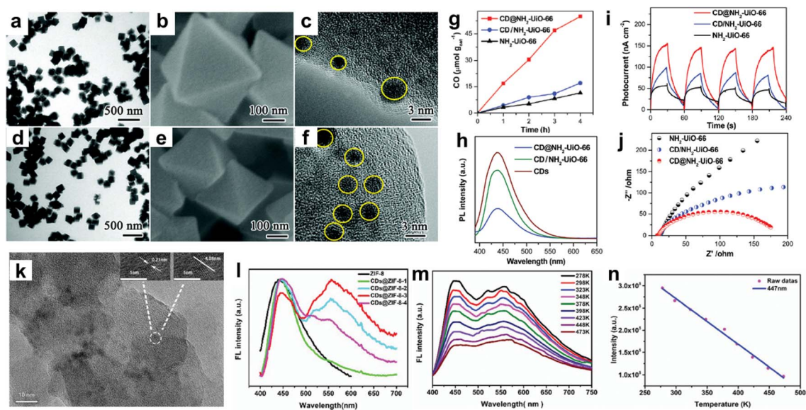
Fig. 3 MOFs–CQD composites prepared through different strategies, namely (a–j) ship-in-bottle and bottle-around-ship, and (k–n) thermal post-synthetic treatment of MOFs loaded with organic molecules. (a–f) TEM and SEM images of (a–c) CQD-decorated UiO-66(Zr)-NH 2 and (d–f) CQD-embedded UiO-66(Zr)-NH 2 . (g–j) characterization of the photocatalytic performance of CQD-embedded UiO-66(Zr)-NH 2 (i.e. CD@NH 2 -UiO-66) in comparison to CQD decorated UiO-66(Zr)-NH 2 (i.e. CD/NH 2 -UiO-66) and pristine UiO-66(Zr)-NH 2 by coupling measurements of (g) the photocatalytic activity for CO 2 reduction, (h) photoluminescence (PL) spectra (i) photocurrents and (j) electrochemical impedance spectra (EIS) (adapted with permission from ref. 30 Copyright 2020, Royal Society of Chemistry). (k) TEM image of CQD@ZIF-8, (l) PL spectra of a series of CQD@ZIF-8 compounds with different CQD loadings, (m) temperature-responsive PL spectra of CQD@ZIF-8, and (n) linear correlation of fluorescence intensity with temperature of CQD@ZIF-8 (emission at 447 nm) (adapted with permission from ref. 38 Copyright 2018, Royal Society of Chemistry).
