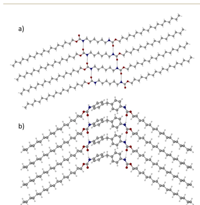
Fig. 4 Crystallographically determined structures of C18-hx (a) and C18-MDP (b). Four molecules are shown to demonstrate the ladder motif formed by the intermolecular hydrogen bonds (represented as broken black lines).
