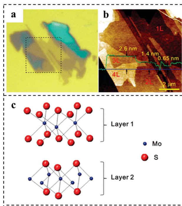
Fig. 10 (a) Optical micrograph of thin \text{MoS}_2 films deposited on the \text{SiO}_2/\text{Si} substrate. (b) AFM height image was taken for the 8 \times 8\ \mu\text{m}^2 area indicated by dotted lines in (a). The thickness of each layer is shown by the height profile (in green) taken along the blue line in the AFM image. (c) Schematic model of the \text{MoS}_2 bilayer structure. Reproduced with permission from ref. 97. Copyright 2010, American Chemical Society.
