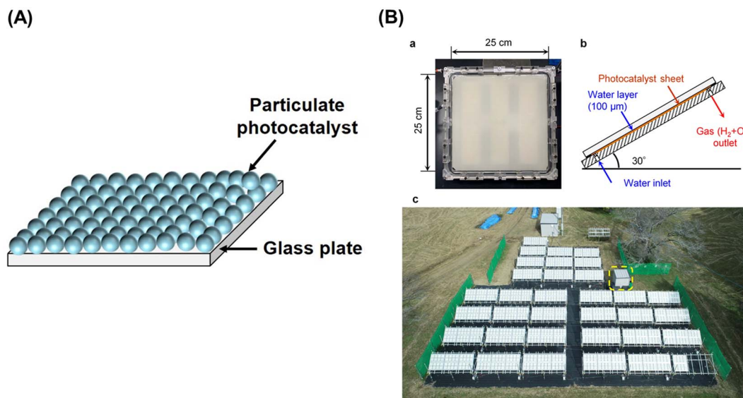
Fig. 2 (A) Schematic diagram of one-step photoexcitation based photocatalyst sheet, (B) 100 m 2 -scale photocatalyst panel reactor: (a) photograph of 625 cm 2 panel reactor unit, (b) schematic side view of panel reactor unit, and (c) top view of 100 m 2 solar hydrogen production system consisting of 1600 panel reactor units. Reproduced from ref. 16 with permission from Springer Nature, copyright 2021.
