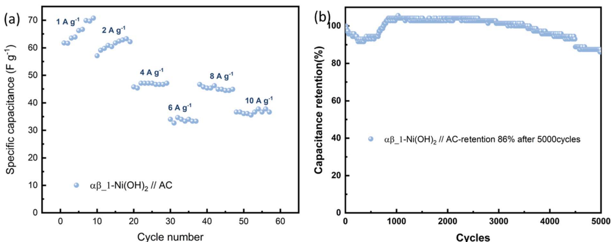
Fig. 11 (a) The specific capacitance evolution under various current densities of \alpha\beta_1 -Ni(OH) 2 //AC. (b) Cycling performance at 100 mA\ cm^{-2} for 5000 cycles.
