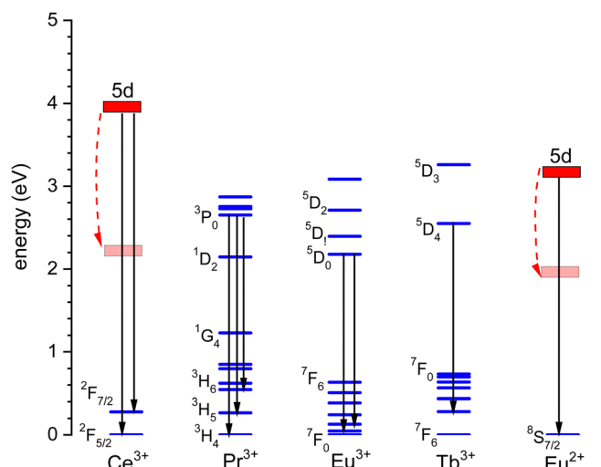
Fig. 2 Relevant level energies and luminescence transitions of \text{Ce}^{3+} , \text{Pr}^{3+} , \text{Eu}^{3+} , \text{Tb}^{3+} , and \text{Eu}^{2+} . The energy of the lowest 5d-level depends on the compound and the range is indicated by the curved dashed arrows.
