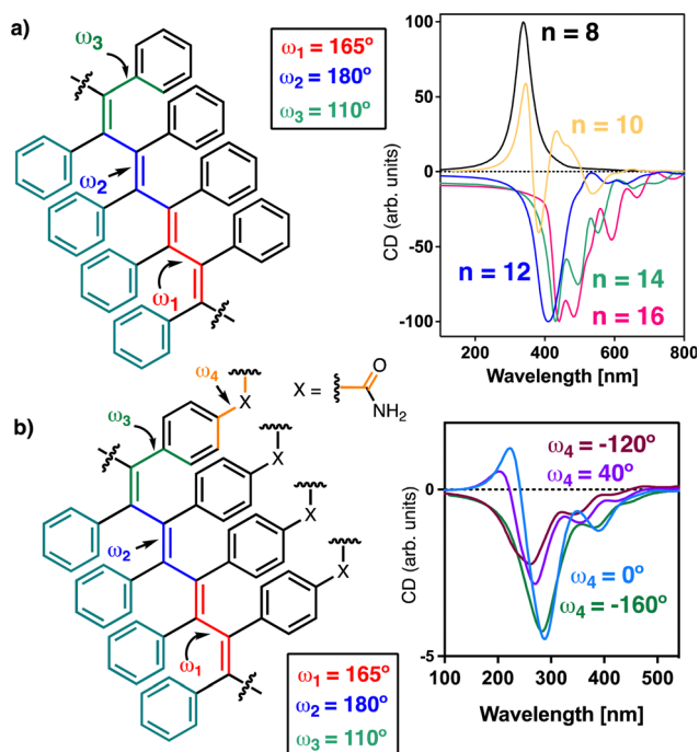
Fig. 3 TD-DFT (CAM-B3LYP)/3-21G ECD spectra of (a) oligomers of different sizes, and (b) a 16-mer with different \omega_4 values. The half width at half height equals (a) 28 nm and (b) 33 nm. For the oligomer structures: \omega_1 = 165^\circ , \omega_2 = 180^\circ and \omega_3 = 110^\circ .
