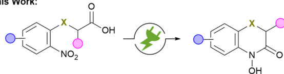
Scheme 2 Conventional and electrochemical reduction of nitroarenes for the synthesis of 2H,4H-4-hydroxy-1,4-benzoxazin-3-ones; C gr = graphite.
