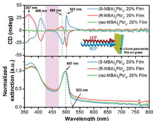
Fig. 4 Transmission CD spectra (above) and normalized extinction spectra (below) of (R/S/Rac\text{-}MBA)_2PbI_4 (in the inset a pictorial representation of a HOIP thin film irradiated by LCP/RCP light). Reprinted with permission from ref. 11 Copyright©2017 Royal Society of Chemistry.
