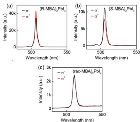
Fig. 5 CPL spectra of (a) (R\text{-}MBA)_2PbI_4 , (b) (S\text{-}MBA)_2PbI_4 and (c) (Rac\text{-}MBA)_2PbI_4 excited by a 473 nm laser at 77 K. Left-handed light, \sigma^- ; right-handed light, \sigma^+ . Reprinted with permission from ref. 21 Copyright©2019 American Chemical Society.
