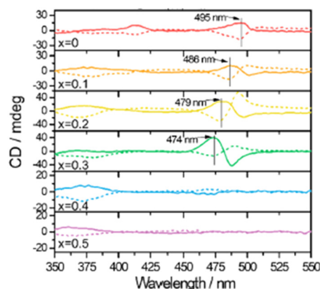
Fig. 6 CD spectra of (R/S\text{-}MBA)_2PbI_{4(1-x)}Br_{4x} . Solid line, S enantiomer; dashed line, R enantiomer. Reprinted with permission from ref. 23 Copyright©2020 American Chemical Society.
