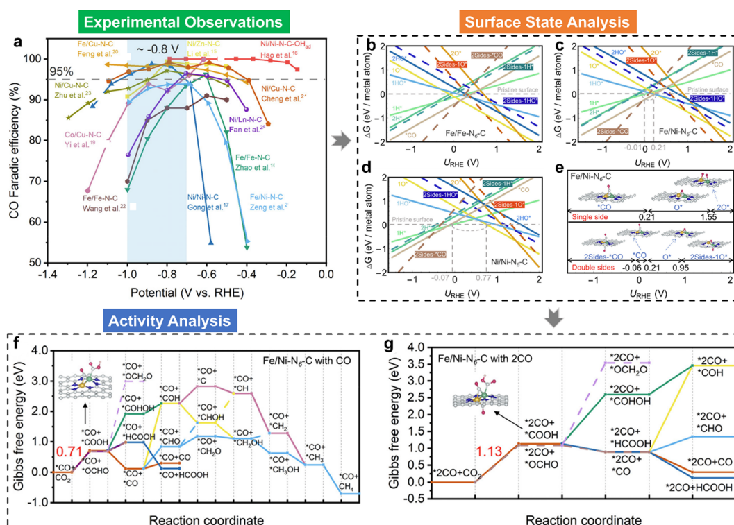
Fig. 6 (a) Comparison of the faradaic efficiency of CO (FE CO ) for various experimentally-reported dual-atom catalysts, where the FE CO data as a function of U_{\text{RHE}} were obtained from their corresponding literatures; calculated 1D surface Pourbaix diagrams of (b) Fe/Fe–N 6 –C, (c) Fe/Ni–N 6 –C, and (d) Ni/Ni–N 6 –C dual-atom catalysts, respectively, where the solid and dashed lines represent single- and double-side adsorption; (e) the surface states of Fe/Ni–N 6 –C at various potential windows, where inserts indicate the atomic configurations; Gibbs free-energy evolutions of the CO 2 RR over Fe/Ni–N 6 –C with pre-covered *CO at (f) single- and (g) double-sides, respectively. 48
