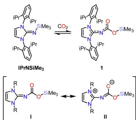
Scheme 1 Top: Equilibrium between IPrNSiMe 3 and 1 . Bottom: Neutral (I) and zwitterionic (II) resonance structures of 1 (R = 2,6-diisopropylphenyl).
