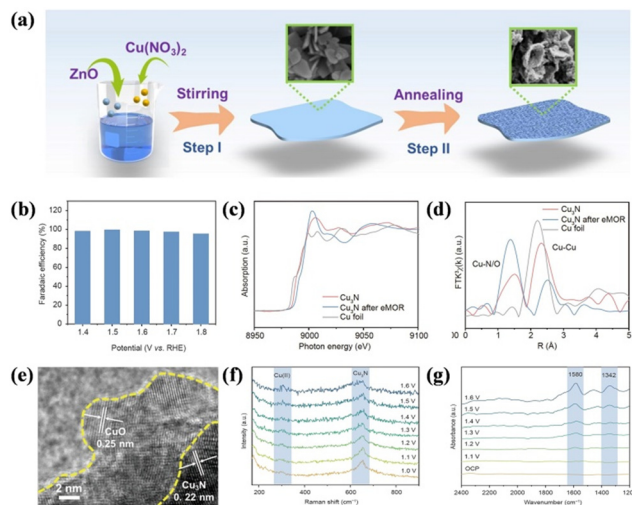
Fig. 10 (a) Schematic of the synthesis of Cu_3N nanosheets. (b) FE of Cu_3N for selective methanol conversion reactions. (c) XANES profiles and (d) FT-EXAFS spectra of Cu foil, Cu_3N , and Cu_3N after eMOR. (e) HRTEM image of Cu_3N after the reaction. (f) In situ Raman spectroscopy and (g) in situ IRAS of Cu_3N electrode. 161 Reproduced from ref. 161 with permission from Springer Nature, Copyright 2023.
