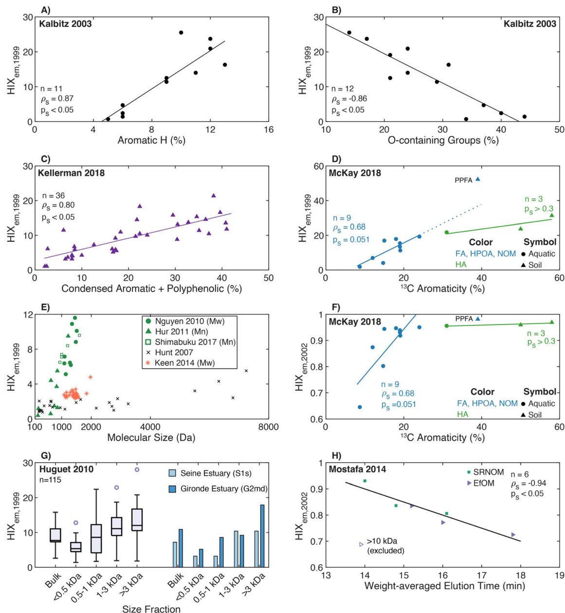
Fig. 9 Relationship between humification index (HIX) and either molecular weight or different measures of aromatic carbon. HIX_{em,1999} versus (A) aromatic proton abundance and (B) oxygen-containing group abundance. 287 (C) HIX_{em,1999} versus the relative abundance of condensed aromatic and polyphenolic formulae (%) per sample calculated by AI_{mod}^{132} from FT-ICR MS data. 35 (D) HIX_{em,1999} versus % aromaticity per sample calculated from ^{13}C NMR pairing optical 39 and NMR data. 40–43 (E) HIX_{em,1999} versus molecular weight determined by SEC and UV detection at 254 nm. 292–296 Legend indicates calculation method ( M_w vs. M_n ) when available. (F) HIX_{em,2002} versus % aromaticity per sample pairing optical 39 and ^{13}C NMR data. 40–43 (G) HIX_{em,1999} versus UF fraction including a boxplot with all data and bar chart with two samples. 297 (H) HIX_{em,2002} vs. weight-averaged elution time from SEC for samples fractionated by UF for a DOM isolate (SRNOM) and wastewater effluent (EfOM). 38 HIX values were not reported in the initial study but calculated from corrected EEMs. Applying a quality control approach, 45 HIX_{em,2002} is not reported for SRNOM in the >10 kDa fraction due to spectral noise. For EfOM, the >10 kDa sample was excluded from the regression.
