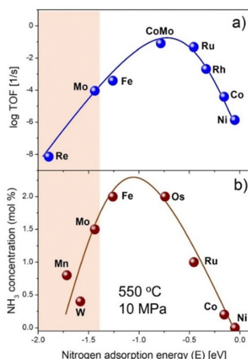
Fig. 1 The classic volcano plot for thermal-catalytic ammonia synthesis. (a) Calculated rate as a function of E_{\text{N}} . (b) The \text{NH}_3 concentration data were taken from ref. 28. The N adsorption energies of Mn and W were taken from ref. 9.
