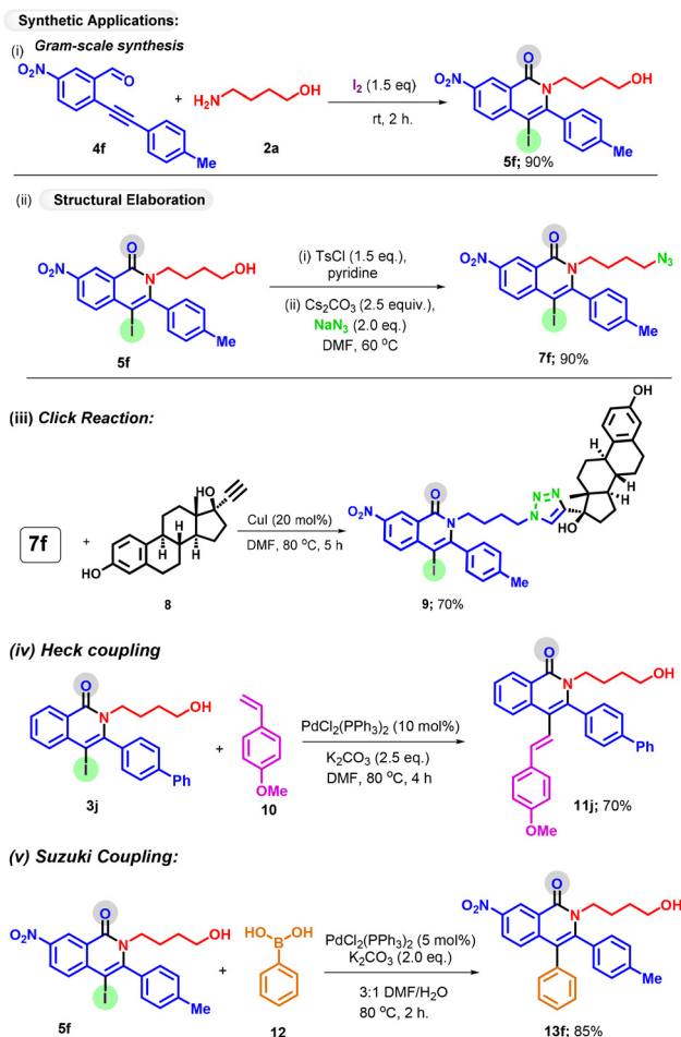
Scheme 5 Synthetic utility of products.
