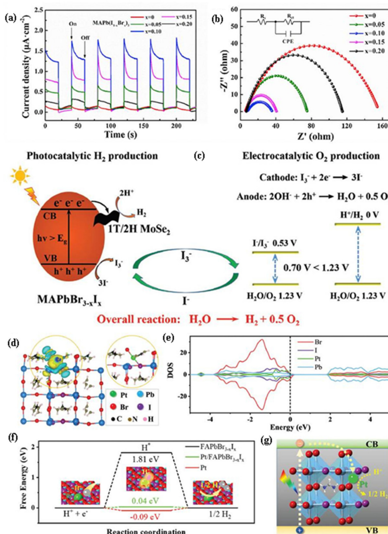
Fig. 13 (a) Chopped photocurrent responses and (b) Nyquist plots of MAPb(I 1-x Br x ) 3 photocatalysts in saturated HI/HBr solution, where x = 0, 0.05, 0.10, 0.15, and 0.20 (reproduced with permission from ref. 2. Copyright 2019, Elsevier B.V.). (c) Schematic diagram depicting the mechanism of pure water splitting using tandem photocatalytic H 2 generation and electrocatalytic O 2 generation with I 3 - /I - as a redox shuttle mediator (reproduced with permission from ref. 10. Copyright 2023, Wiley-VCH GmbH). (d) The difference in the charge densities of Pt/FAPbBr 3-x I x , where the inset depicts its local structure, while the isosurface value is set at 0.001 e Å -3 (positive charge: yellow color; negative charge: cyan color); (e) projected density of states (PDOS) of the photocatalyst (Pt/FAPbBr 3-x I x ); (f) calculated free energy of H + adsorption on Pt/FAPbBr 3-x I x in comparison with those of Pt and FAPbBr 3-x I x , where the inset depicts the corresponding schematic mechanism; (g) schematic diagram illustrating the photocatalytic process for Pt/FAPbBr 3-x I x (reproduced with permission from ref. 32. Copyright 2022, The Royal Society of Chemistry).
