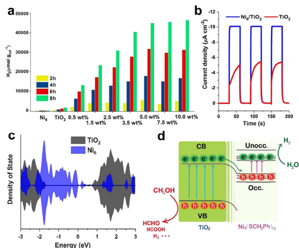
Fig. 7 (a) Photocatalytic \text{H}_2 production performance of catalysts with different cluster loadings in a mixture of distilled water and methanol ( v/v = 80 \text{ mL}/20 \text{ mL} ) with simulated solar light irradiation powered by a 300 W Xe lamp. (b) Photo-response currents of \text{Ni}_6/\text{TiO}_2 and \text{TiO}_2 . (c) Electron density states of pristine \text{TiO}_2 and \text{Ni}_6 cluster. (d) Schematic diagram of the mechanism of photogenerated electron-hole pair transfer between \text{TiO}_2 and \text{Ni}_6 clusters. Reproduced with permission from ref. 75. Copyright 2021 Elsevier.
