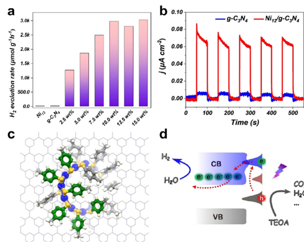
Fig. 8 (a) Photocatalytic \text{H}_2 production efficiency of catalysts with different \text{Ni}_{12} cluster loadings in a mixture of distilled water and methanol ( v/v = 80 \text{ mL}/20 \text{ mL} ) with simulated solar light irradiation powered by a 300 W Xe lamp. (b) Photo-response currents of \text{Ni}_{12}/\text{g-C}_3\text{N}_4 and \text{g-C}_3\text{N}_4 . (c) Ab initio molecular dynamic snapshots of \text{Ni}_{12} loaded onto \text{g-C}_3\text{N}_4 systems at 10 ps. Color codes: blue = Ni, yellow = S, grey = C, white = H. (d) Schematic diagram of the mechanism of photogenerated electron-hole pair transfer between \text{g-C}_3\text{N}_4 and \text{Ni}_{12} clusters. Reproduced with permission from ref. 76. Copyright 2023 American Chemical Society.
