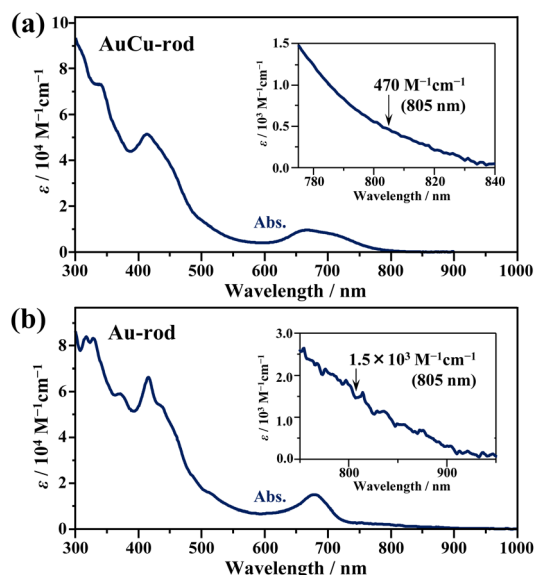
Fig. 1 Absorption spectra of (a) AuCu-rod and (b) Au-rod in tetrahydrofuran. The insets display expanded views of the absorption edge region, together with the molar absorption coefficients of the nanoclusters at the excitation light of 805 nm used in the upconversion measurements.
