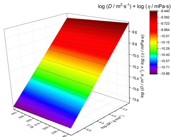
Fig. 3 3D calibration fit of viscosity-corrected diffusion coefficients (obtained using dstepbpgp3s) as a function of temperature and the molar mass of polystyrene standards.
