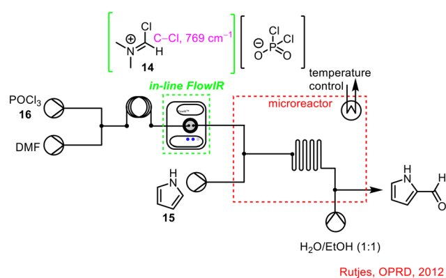
Scheme 5 In-line FlowIR flow cell used to monitor conversion of POCl 3 16 in the telescoped process to synthesise 2-formylpyrrole 17 (ref. 43).
