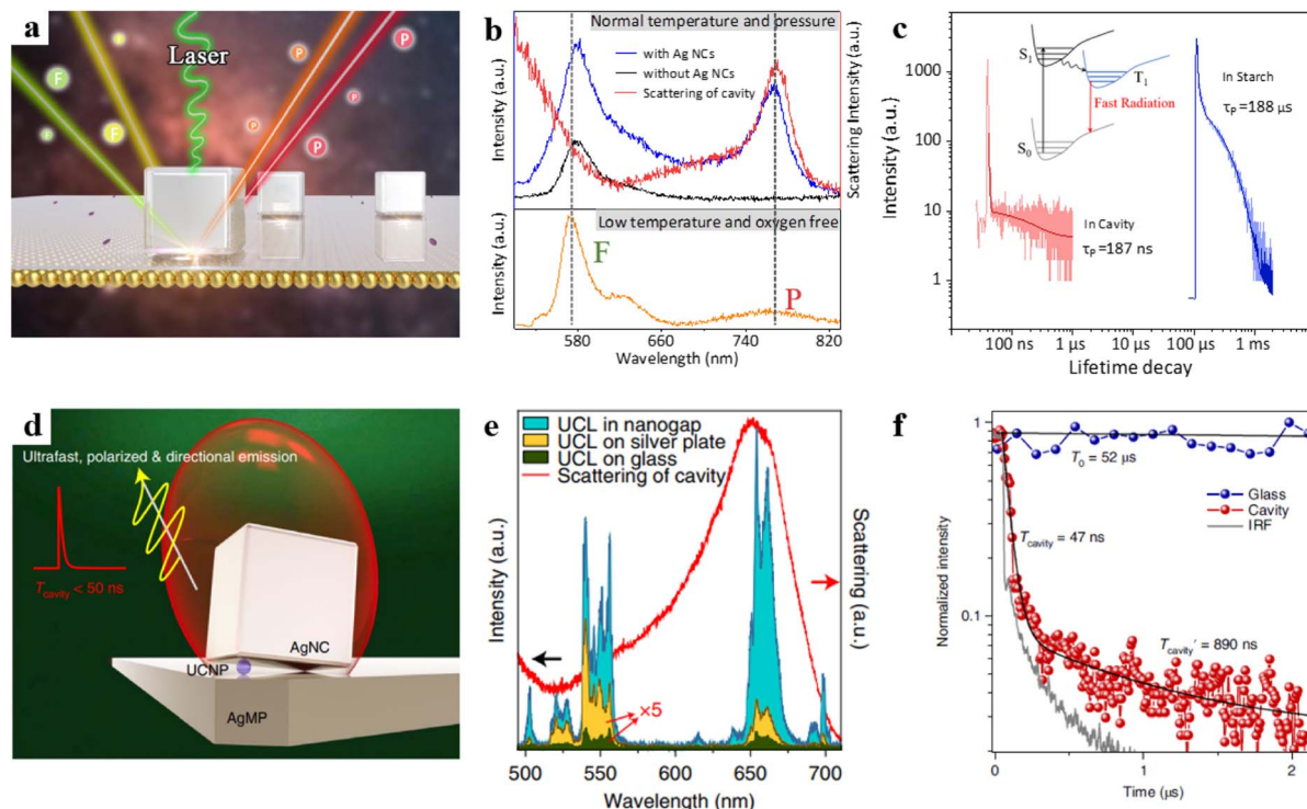
Fig. 6 (a) Schematic diagram of the model. (b) The bottom panel is the emission spectrum of the RB at -190^\circ C under hypoxic conditions, the top panel is the emission spectra of the Au film surface with RB probe molecules at room temperature and the corresponding dark-field scattering spectrum. (c) Transient dynamics of RB in optical cavities and in starch. Panels (a)–(c) are reprinted with permission from ref. 97, Copyright from 2023, American Chemical Society. (d) Schematic of the tilted-nanocavity-coupled UCNP. (e) Upconversion luminescence spectra and the dark-field scattering spectrum. (f) Normalized transient dynamics of UCNPs in the tilted cavity and on the glass slide. Panels (d)–(f) are reprinted with permission from ref. 43, Copyright from 2022, Springer Nature Limited.
