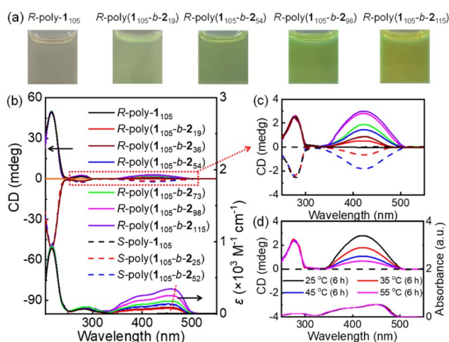
Fig. 4 (a) Photographs of R -poly( 1_{105} - b - 2_n ) copolymers under room light in THF. (b) CD and UV-vis absorption spectra of poly( 1_{105} - b - 2_n ) copolymers (THF, 25 °C). (c) Amplified CD spectra of poly( 1_{105} - b - 2_n ) copolymers (THF, 25 °C). (d) CD and UV-vis absorption spectra of poly( 1_{105} - b - 2_n ) copolymers measured in THF at different temperatures.
