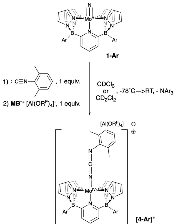
Scheme 6 Reaction of 1-Ar with 1 equivalent of oxidant at -78^\circ\text{C} in the presence of xyl isocyanide.
