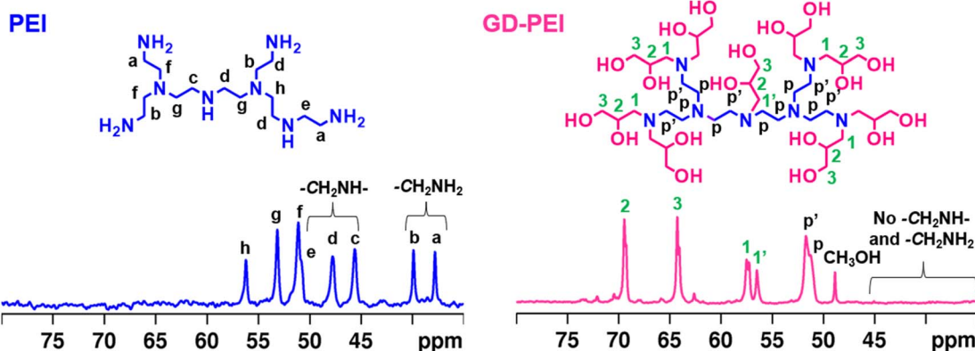
Fig. 4 ^{13}C NMR spectra of PEI and GD-PEI.
