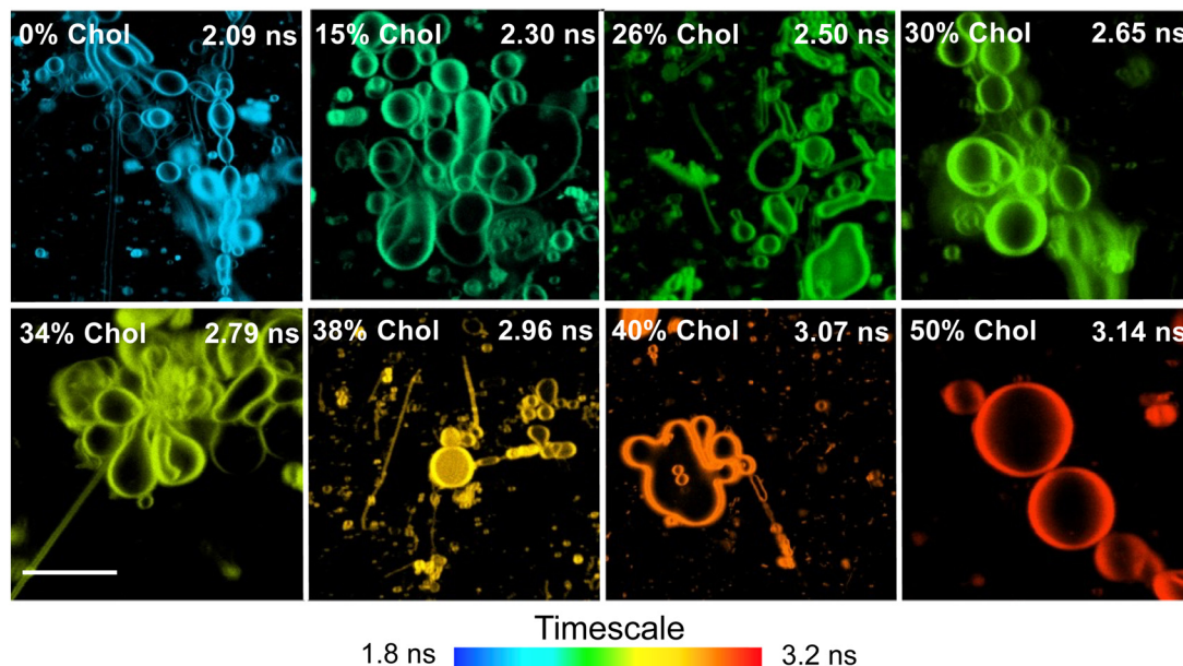
Fig. 2 Representative FLIM images for DI-8-ANEPPS-intercalated POPC:POPG GMLVs with different cholesterol levels. The scale bar is 10 \mu m.
