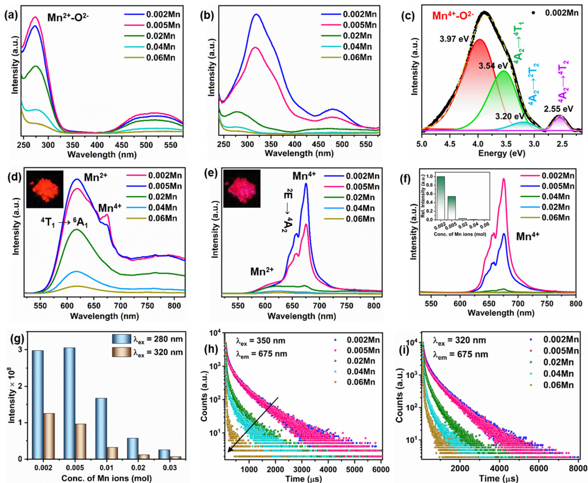
Fig. 1 PLE spectra of YAGG: x Mn ( x = 0.002 – 0.06 mol) phosphors monitored at (a) \lambda_{em} = 620 nm and (b) \lambda_{em} = 675 nm. (c) Deconvolution of the PLE spectrum of YAGG:0.002Mn monitored at 675 nm. PL emission spectra for (d) \lambda_{ex} = 280 nm and (e) \lambda_{ex} = 320 nm (emission photograph of YAGG:0.002Mn in inset). (f) PL emission spectra for \lambda_{ex} = 350 nm (inset showing the relative intensity with increasing Mn doping amounts). (g) Integral intensity as a function of Mn ions concentration. (h) Decay curves of Mn^{4+} ions at \lambda_{ex} = 350 nm and \lambda_{em} = 675 nm. (i) Decay curves of Mn ions at \lambda_{ex} = 320 nm and \lambda_{em} = 675 nm.
