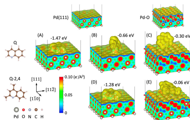
Fig. 5 Adsorption energy and structure of quinoline (Q) on (A) and (B) Pd(111) and (C) PdO surface and 2,4-dimethylquinoline (Q-2,4) on (D) Pd(111) and (E) PdO surface. Charge density isosurface of 0.005 e − Å −3 is shown.
