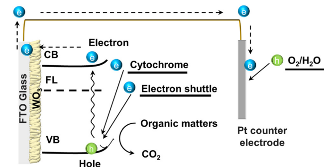
Fig. 5 Schematic diagram of the photocurrent generation by the \text{WO}_3 electrode with MR-1 bacteria. FL, CB, and VB represent the fermi level, conduction, and valence bands, respectively.
