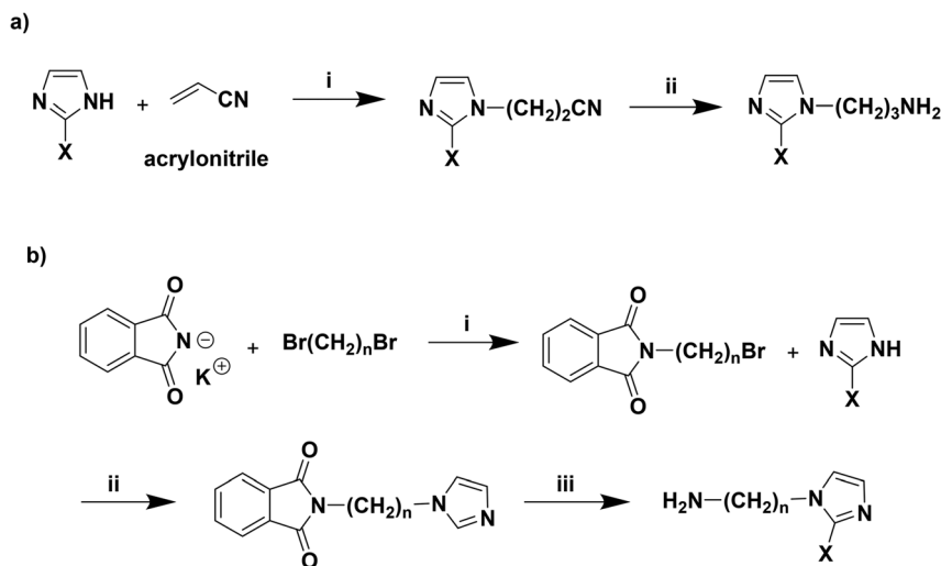
Scheme 2 a) (i) Imidazole and acrylonitrile in presence of Et 3 N and toluene produce imidazole-propylnitrile, (ii) reduction to API by H 2 in the presence of RANEY® nickel catalyst in aqueous MeOH/NH 4 OH. (b) (i) Phthalimide potassium salt reacting with dibromo-alkane in DMF at 100 °C 24 h to produce N -(ω-bromoalkyl) phthalimide, (ii) reaction with imidazole compound in DMF at 80 °C for 8 h to produce the imidazole-tethered-phthalimide, (iii) removal of protecting group to obtain corresponding 1-(ω-aminoalkyl) imidazole with hydrazine hydrate in EtOH for 24 h at reflux.
