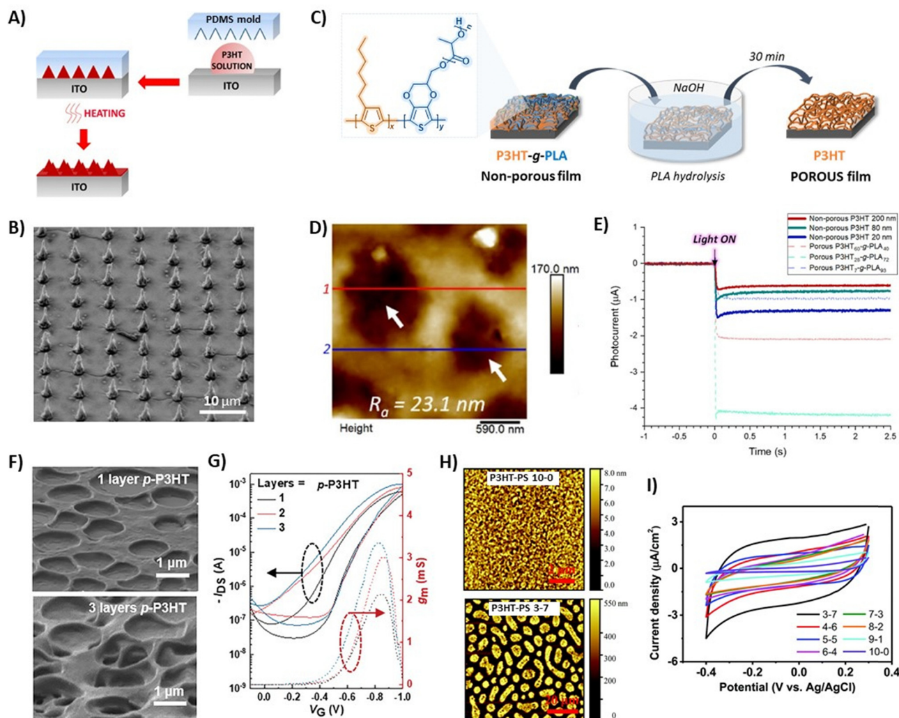
Fig. 4 (A) Schematic representation of the P3HT micropillar fabrication process by moulding, and (B) SEM image of P3HT pillar structure. Reprinted with permission. 55 Copyright 2019 American Chemical Society. (C) Schematic representation of the fabrication of porous thin films by PLA hydrolysis; (D) topographical AFM image of a representative porous P3HT film after PLA hydrolysis of P3HT 60 -g-PLA 40 copolymer film; and (E) photocurrent curves of non-porous P3HT films with different thicknesses and porous films made of P3HT x -g-PLA y copolymers when irradiated with a LED (530 nm, 110 mW cm -2 ). Reprinted with permission. 57 Copyright 2023 American Chemical Society. (F) SEM images of porous P3HT/SEBS films, and (G) transfer curves and corresponding g_m evolutions for OECTs based on multilayers of P3HT. Reprinted with permission. 58 Copyright 2023 Wiley-VCH GmbH. (H) AFM images of porous P3HT films obtained from phase separation P3HT/PS followed by dissolution of PS by washing with acetone, and (I) CV scans (100 mV s -1 ) of the O 2 plasma-treated porous P3HT films. Reprinted with permission. 59 Copyright 2020 The Royal Society of Chemistry.
