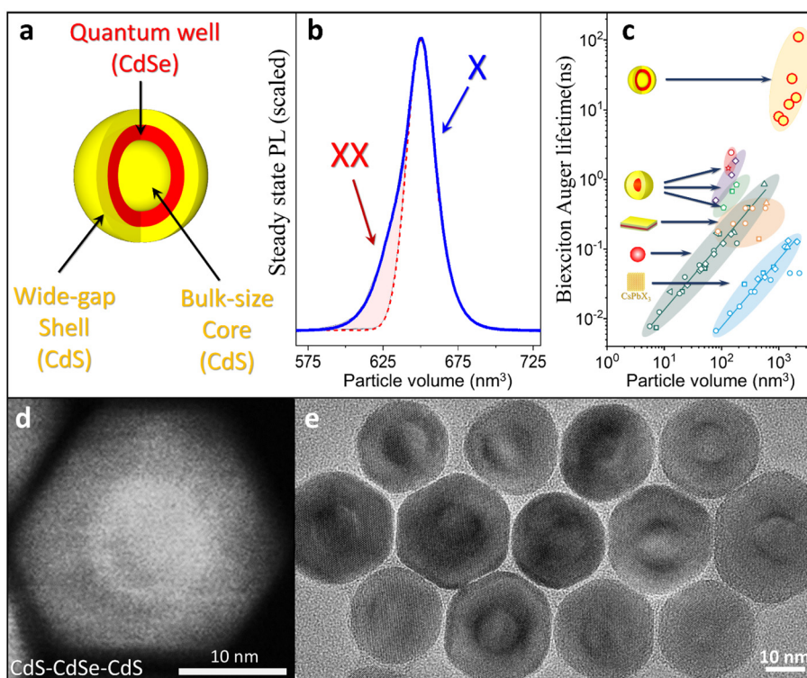
Fig. 1 (a) The schematic geometry of a \text{CdS}_{\text{bulk}}\text{-CdSe-CdS} QS. (b) Steady-state PL of \text{CdS-CdSe-CdS} QDs showing the contribution from biexciton emission on the high energy side of single-exciton PL peak. (c) The dependence of biexciton Auger lifetimes on particle volume for different types of colloidal NCs. (d) Characteristic high angle annular dark field (HAADF)-STEM image of a \text{CdS-CdSe-CdS} QS, illustrating the location of the CdSe shell layer. (e) Characteristic TEM image of 14 nm-core \text{CdS-CdSe-CdS} QDs. Adapted with permission from ref. 34. Copyright 2023 The Royal Society of Chemistry. Panel c adapted with permission from ref. 42. Copyright 2021. Springer Nature.
