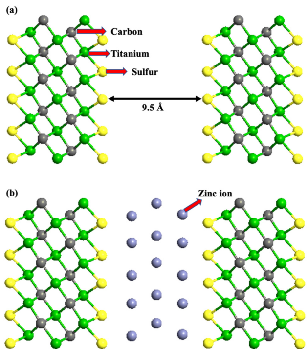
Fig. 2 Side view of (a) the optimized structure of the b \text{Ti}_3\text{C}_2\text{-S}_2 MXene before Zn-ion intercalation and (b) the optimized structure of the b \text{Ti}_3\text{C}_2\text{-S}_2 MXene after Zn-ion intercalation.
