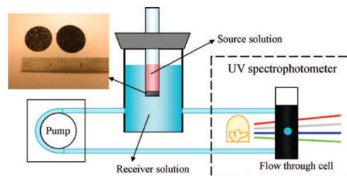
Fig. 16 Schematic setup used by Hou et al. 176 Reproduced from ref. 176 with permission from ACS, copyright 2025.
