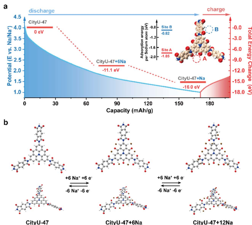
Fig. 6 DFT calculations. (a) Proposed sodiation pathway of the CityU-47 electrode, with redox potential vs. \text{Na}/\text{Na}^+ on the left axis and total energy change on the right axis. (b) The corresponding structural evolution of CityU-47 during the sodiation procedure.
