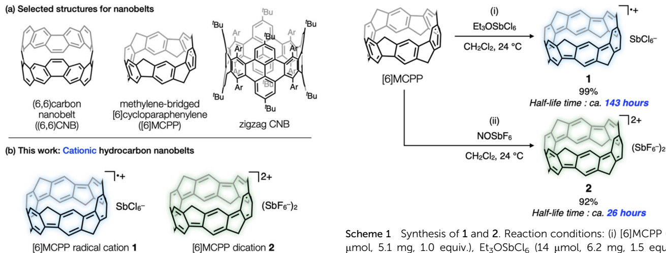
Fig. 1 (a) The structures of neutral aromatic hydrocarbon nanobelts. Ar = p - ^t\text{BuC}_6\text{H}_4 . (b) The structures of [6]MCPP radical cation \text{SbCl}_6^- salt 1 and [6]MCPP dication ( \text{SbF}_6^- ) 2 salt 2 .
